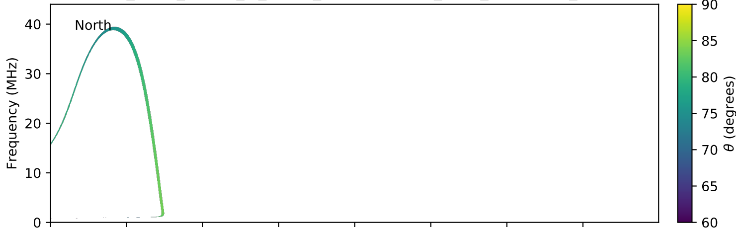
expres_earth_jupiter_io_jrm09_lossc-wid1deg_3kev_20161012_v01.cdf
