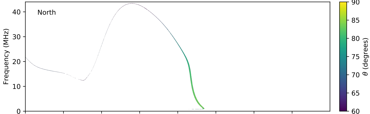
expres_earth_jupiter_io_jrm09_lossc-wid1deg_3kev_20161008_v01.cdf
