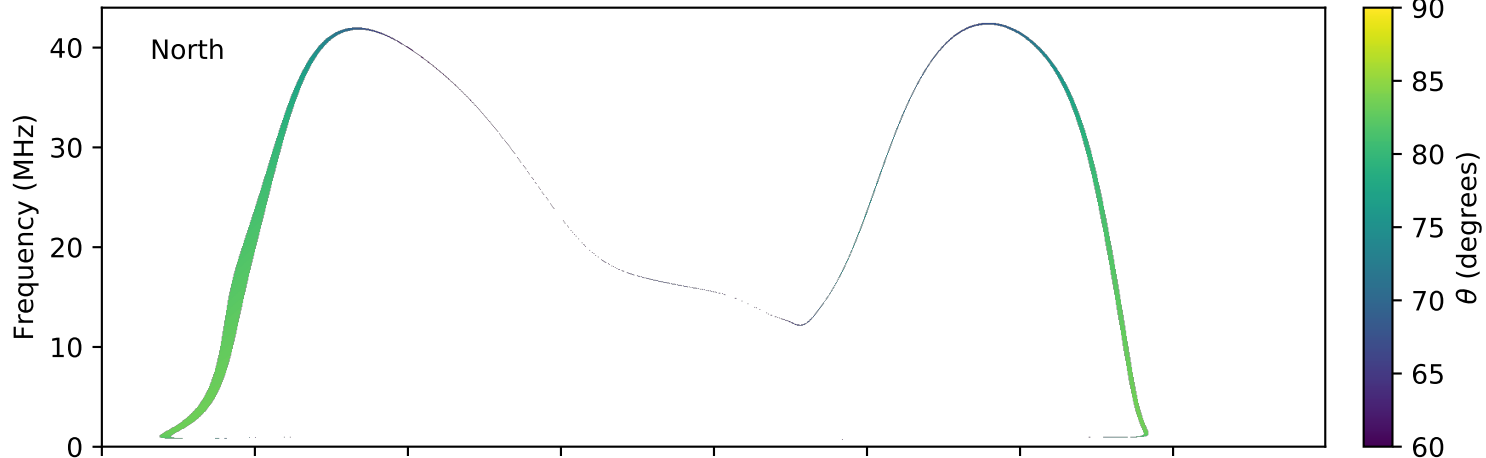
expres_earth_jupiter_io_jrm09_lossc-wid1deg_3kev_20161006_v01.cdf
