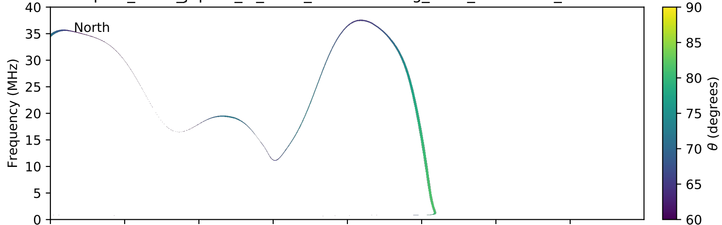
expres_earth_jupiter_io_isaac_lossc-wid1deg_5kev_20161031_v01.cdf
