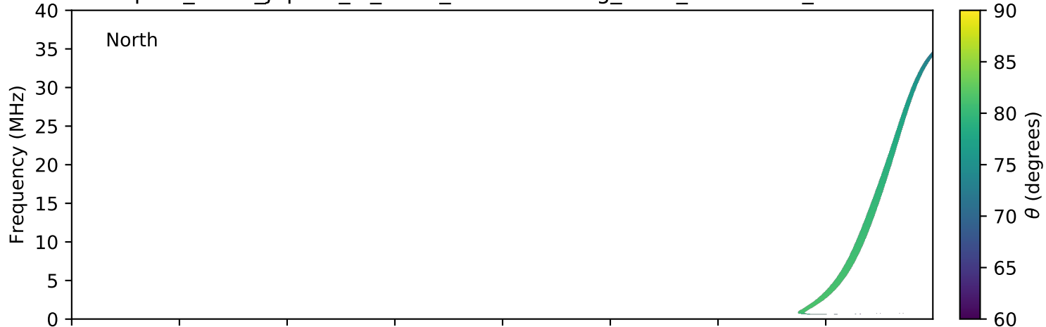
expres_earth_jupiter_io_isaac_lossc-wid1deg_5kev_20161030_v01.cdf
