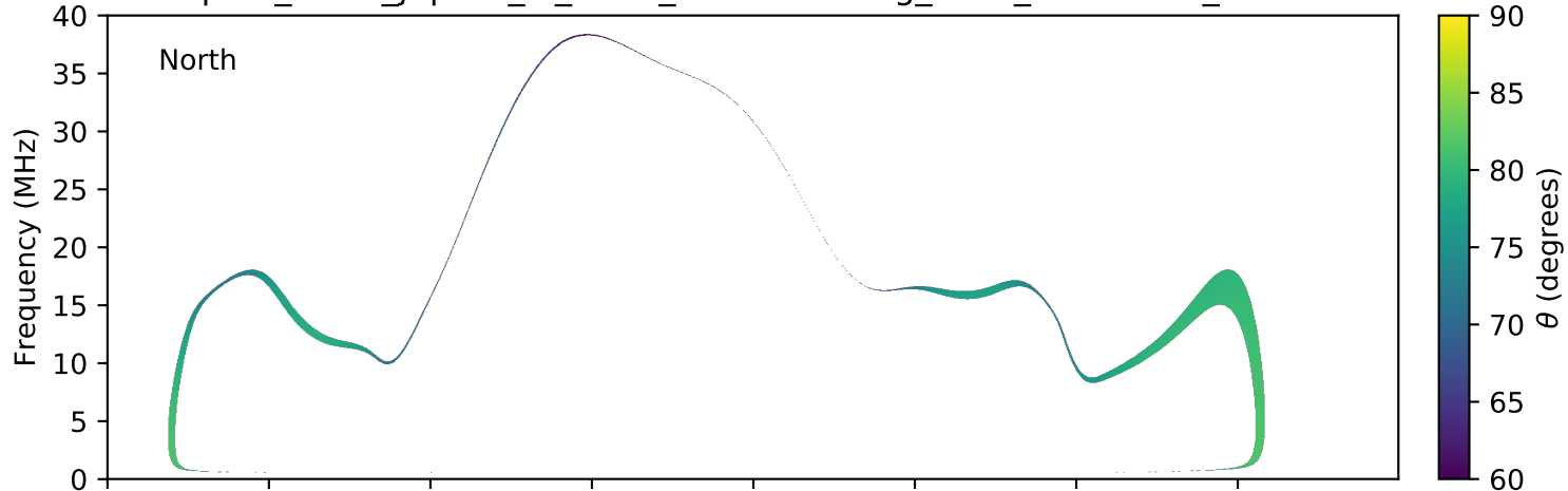
expres_earth_jupiter_io_isaac_lossc-wid1deg_5kev_20161029_v01.cdf
