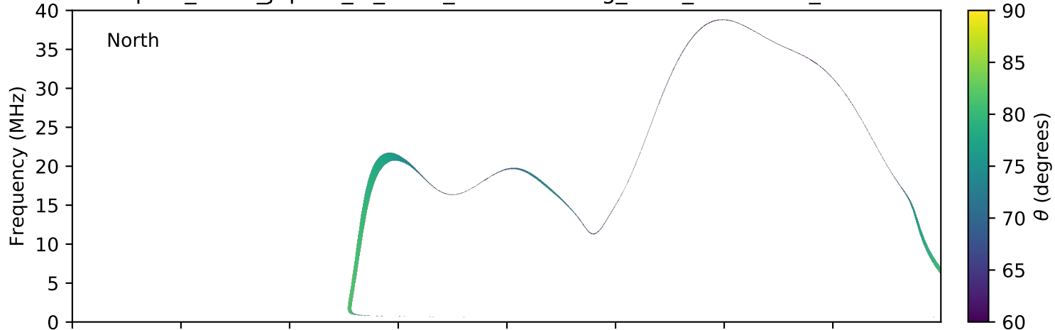
expres_earth_jupiter_io_isaac_lossc-wid1deg_5kev_20161027_v01.cdf
