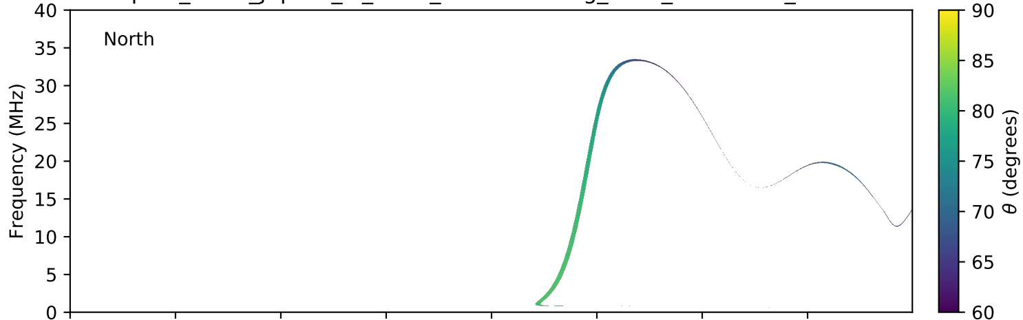
expres_earth_jupiter_io_isaac_lossc-wid1deg_5kev_20161025_v01.cdf
