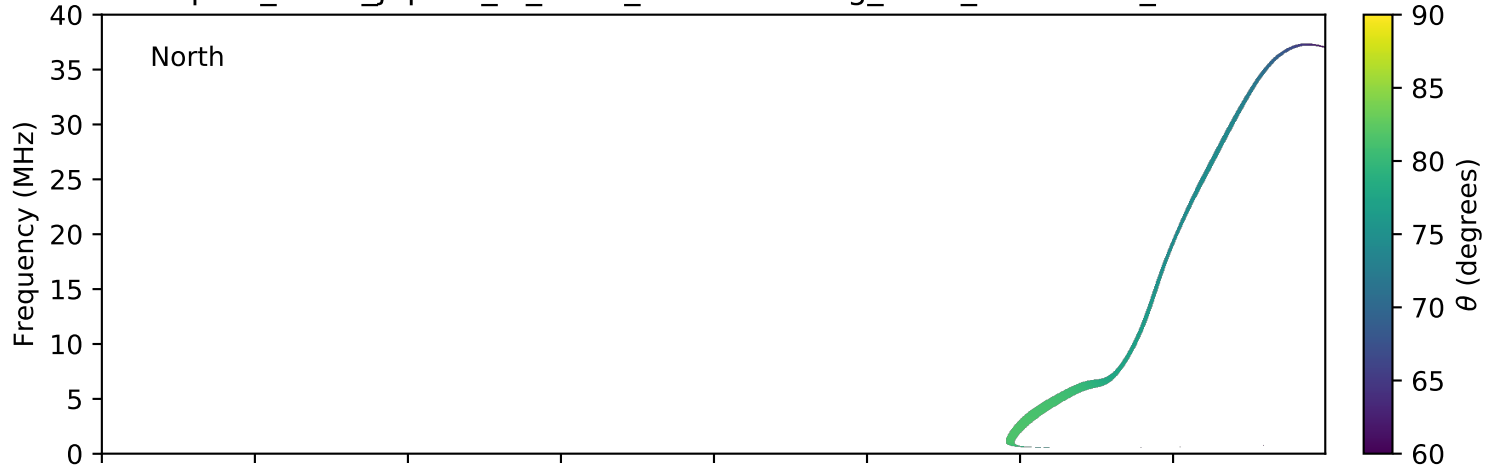
expres_earth_jupiter_io_isaac_lossc-wid1deg_5kev_20161023_v01.cdf
