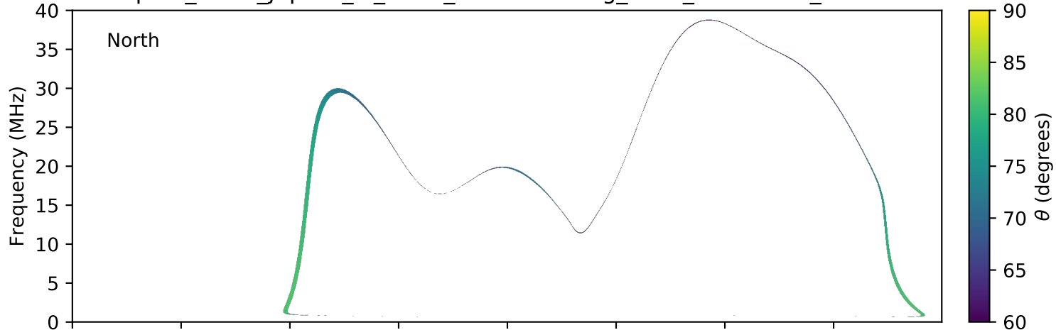
expres_earth_jupiter_io_isaac_lossc-wid1deg_5kev_20161020_v01.cdf
