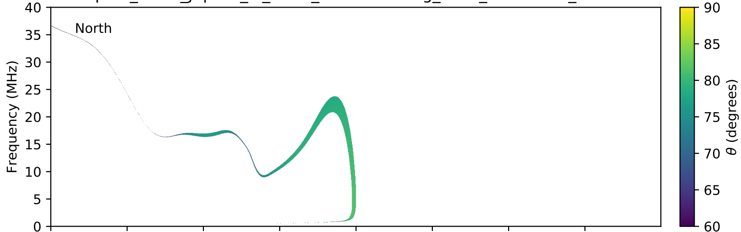
expres_earth_jupiter_io_isaac_lossc-wid1deg_5kev_20161017_v01.cdf
