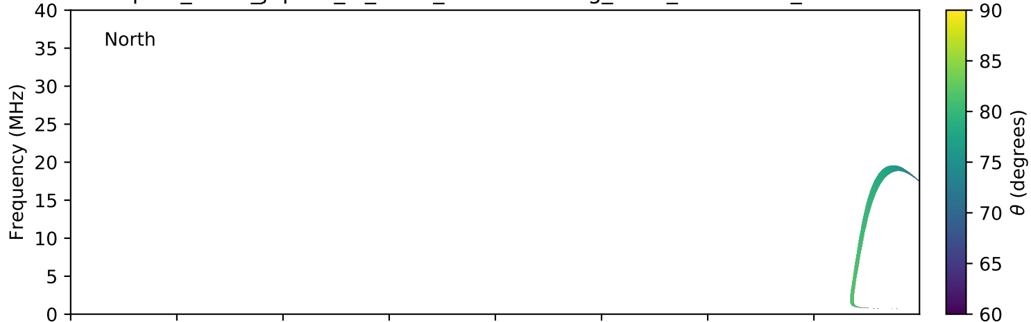
expres_earth_jupiter_io_isaac_lossc-wid1deg_5kev_20161014_v01.cdf
