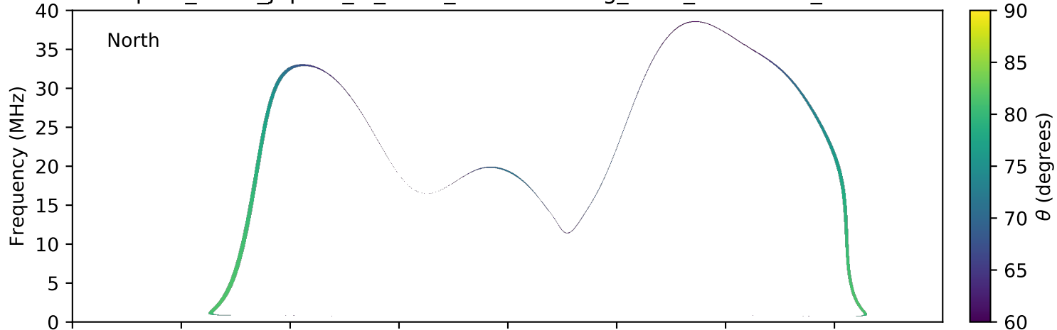
expres_earth_jupiter_io_isaac_lossc-wid1deg_5kev_20161013_v01.cdf
