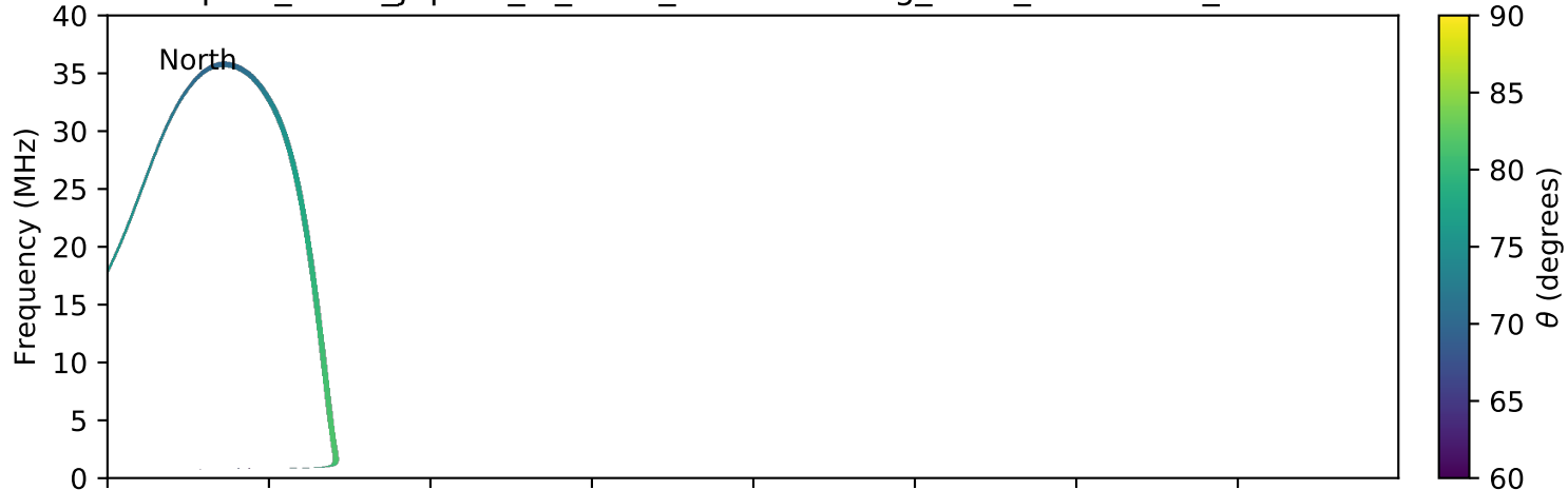
expres_earth_jupiter_io_isaac_lossc-wid1deg_5kev_20161012_v01.cdf
