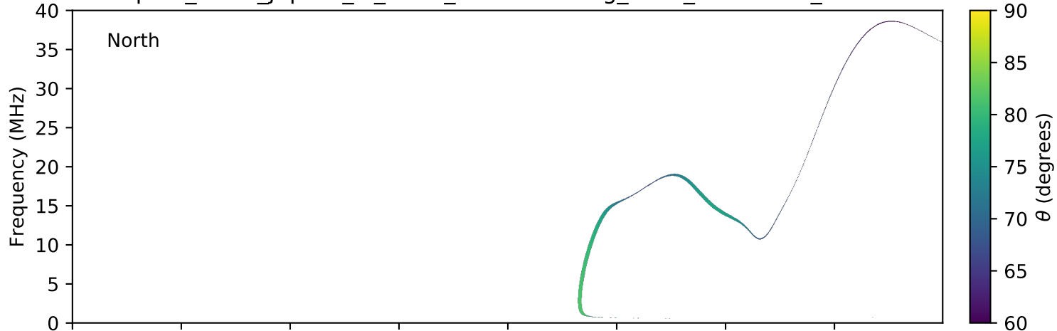
expres_earth_jupiter_io_isaac_lossc-wid1deg_5kev_20161009_v01.cdf
