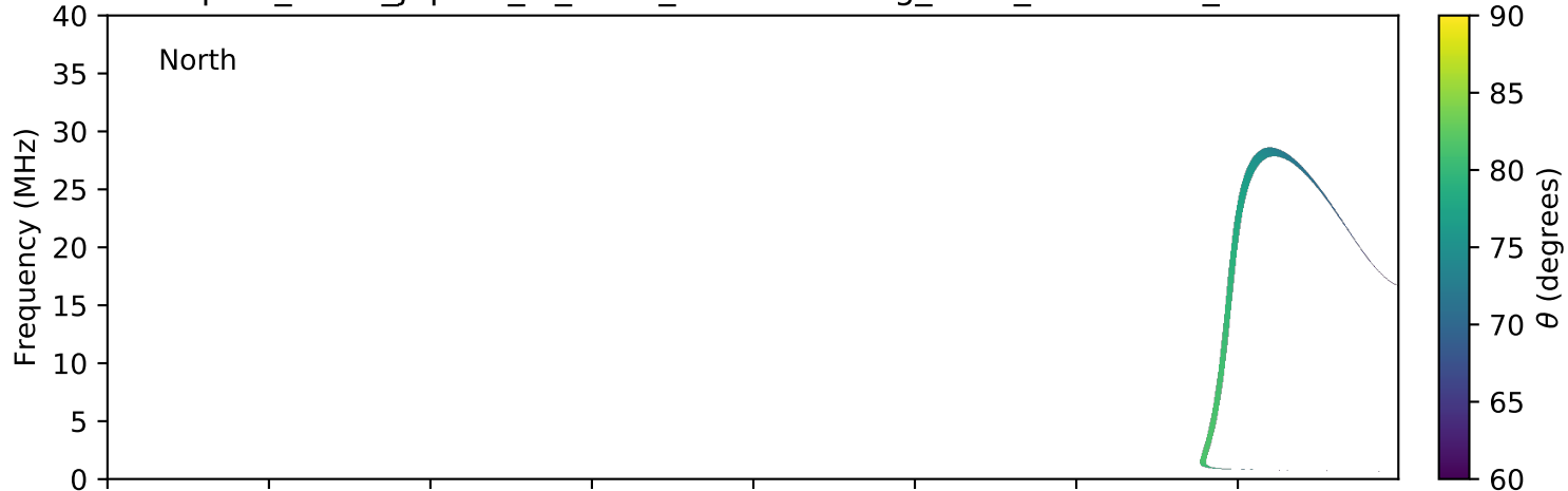
expres_earth_jupiter_io_isaac_lossc-wid1deg_5kev_20161007_v01.cdf
