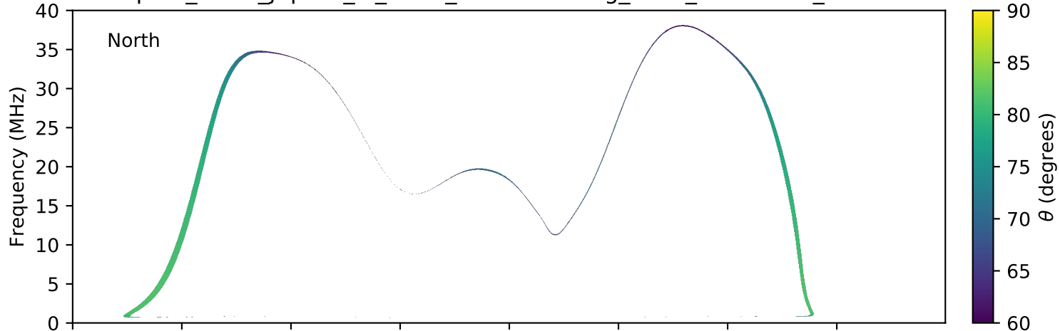
expres_earth_jupiter_io_isaac_lossc-wid1deg_5kev_20161006_v01.cdf
