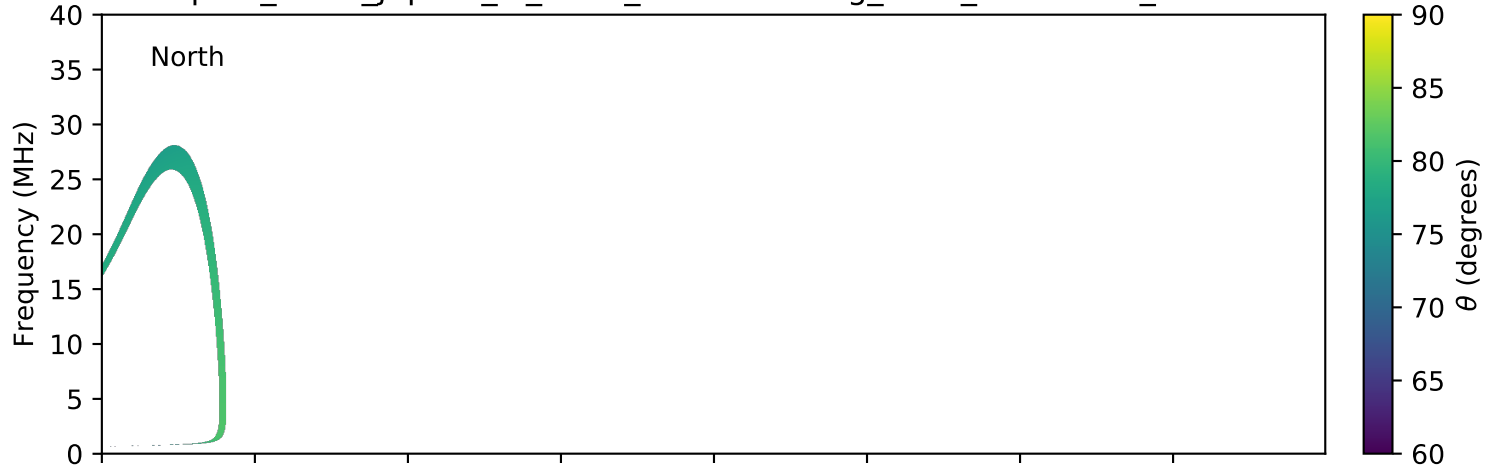
expres_earth_jupiter_io_isaac_lossc-wid1deg_5kev_20161005_v01.cdf
