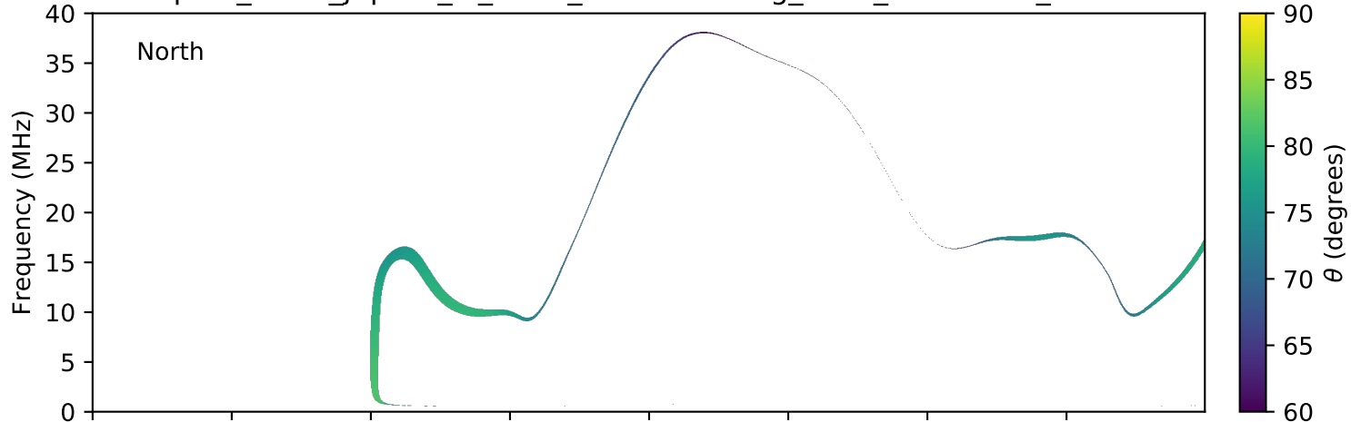
expres_earth_jupiter_io_isaac_lossc-wid1deg_5kev_20161004_v01.cdf
