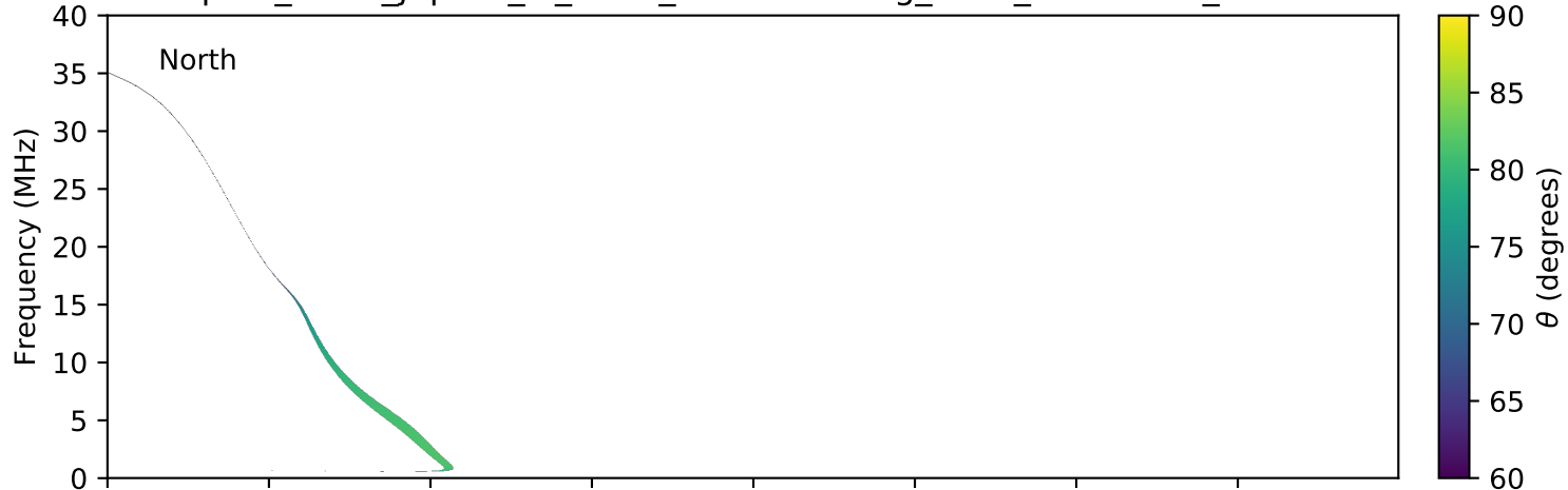
expres_earth_jupiter_io_isaac_lossc-wid1deg_5kev_20161003_v01.cdf
