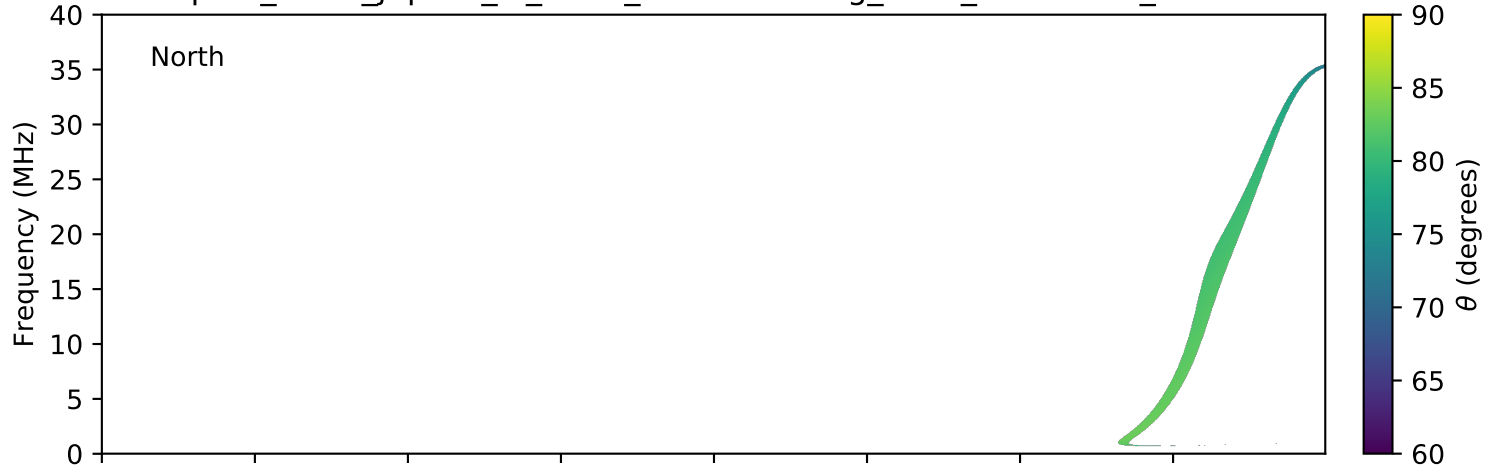
expres_earth_jupiter_io_isaac_lossc-wid1deg_3kev_20161030_v01.cdf
