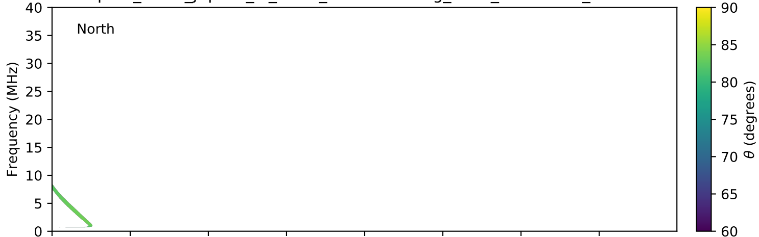
expres_earth_jupiter_io_isaac_lossc-wid1deg_3kev_20161028_v01.cdf
