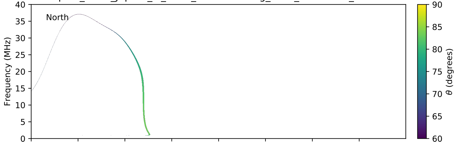
expres_earth_jupiter_io_isaac_lossc-wid1deg_3kev_20161026_v01.cdf
