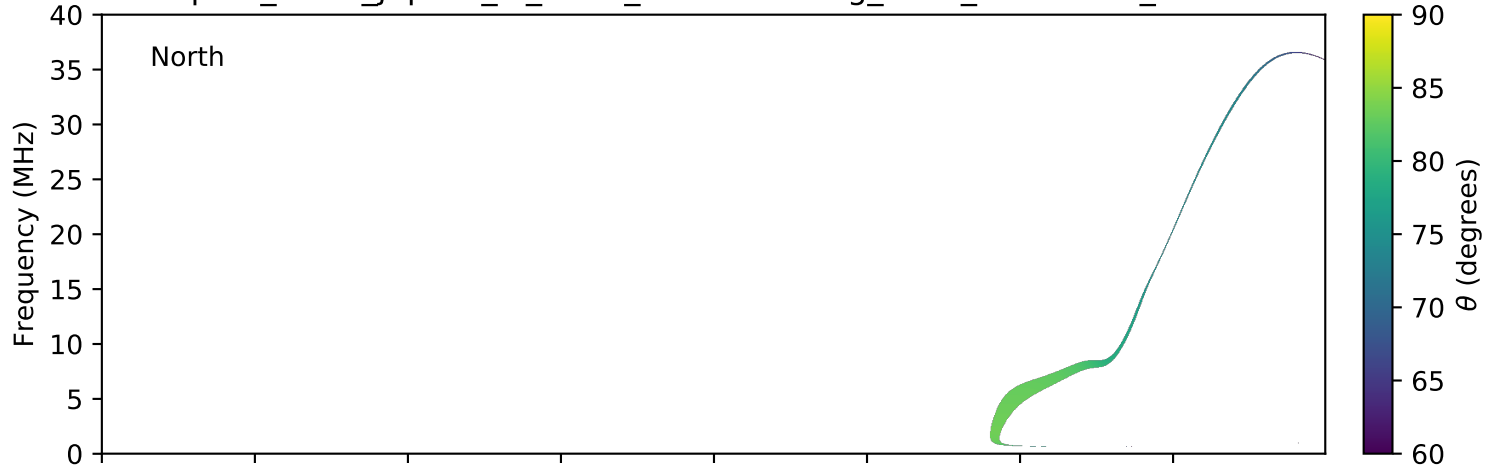
expres_earth_jupiter_io_isaac_lossc-wid1deg_3kev_20161023_v01.cdf
