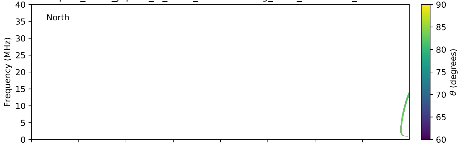
expres_earth_jupiter_io_isaac_lossc-wid1deg_3kev_20161021_v01.cdf
