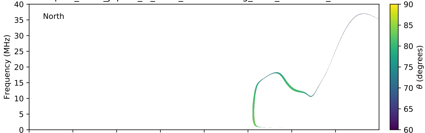
expres_earth_jupiter_io_isaac_lossc-wid1deg_3kev_20161016_v01.cdf
