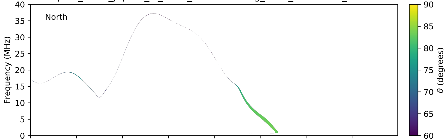
expres_earth_jupiter_io_isaac_lossc-wid1deg_3kev_20161015_v01.cdf
