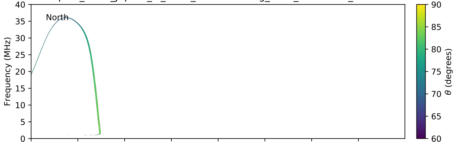
expres_earth_jupiter_io_isaac_lossc-wid1deg_3kev_20161012_v01.cdf
