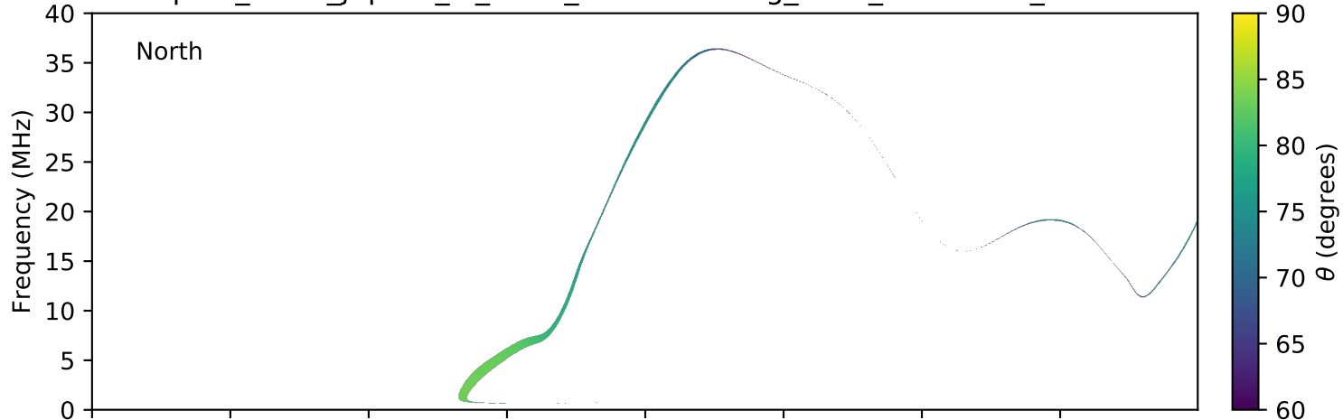
expres_earth_jupiter_io_isaac_lossc-wid1deg_3kev_20161011_v01.cdf
