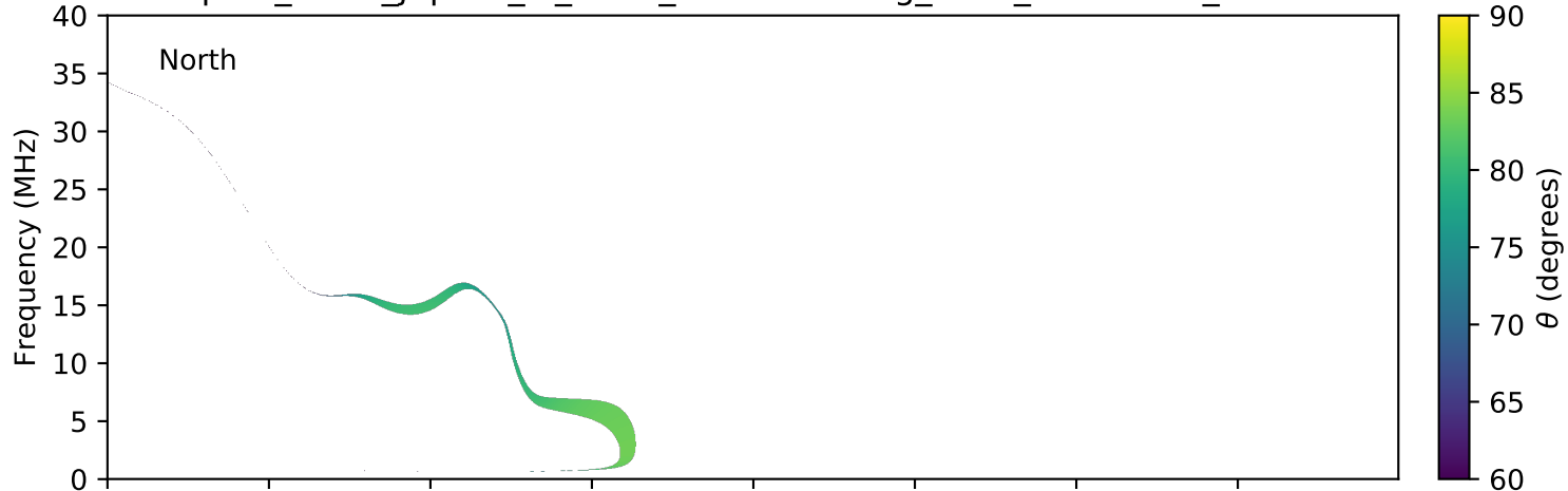
expres_earth_jupiter_io_isaac_lossc-wid1deg_3kev_20161010_v01.cdf
