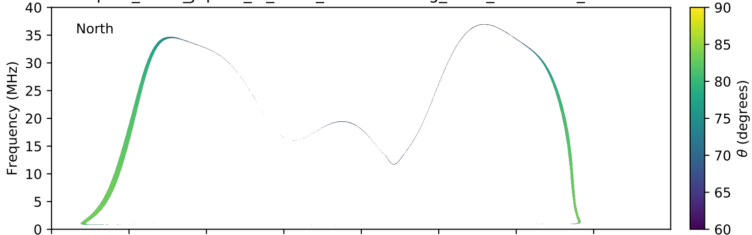
expres_earth_jupiter_io_isaac_lossc-wid1deg_3kev_20161006_v01.cdf
