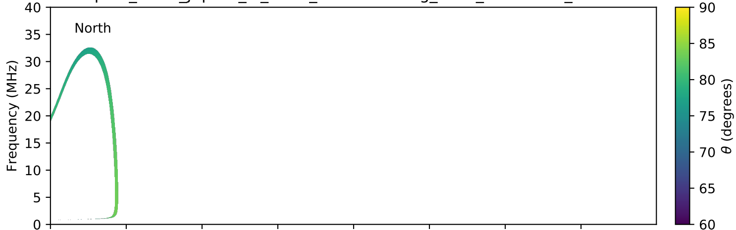
expres_earth_jupiter_io_isaac_lossc-wid1deg_3kev_20161005_v01.cdf
