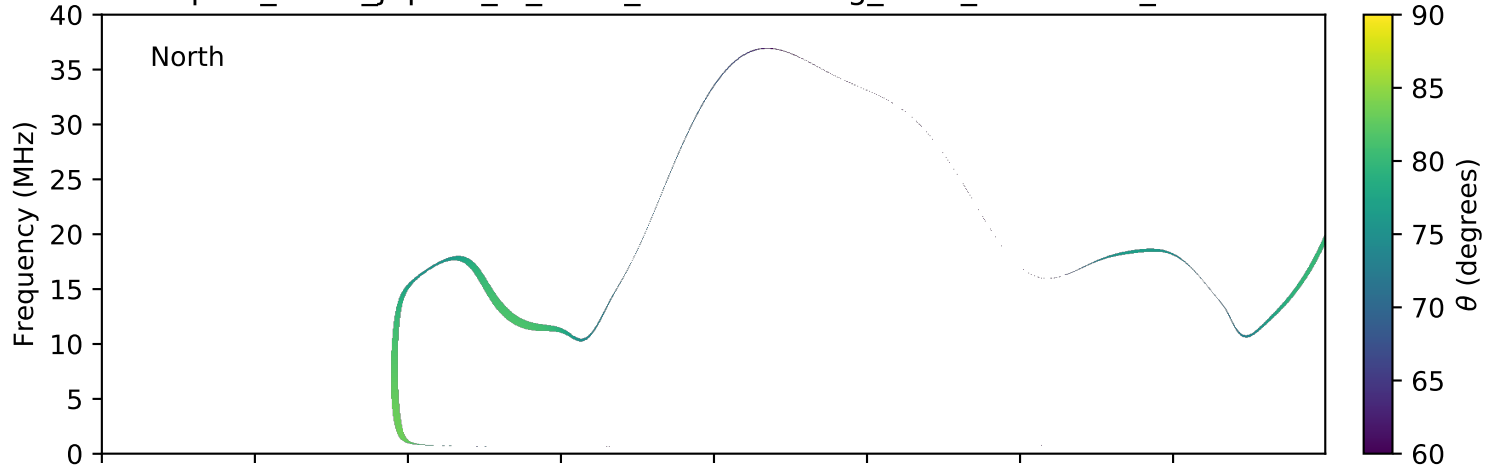
expres_earth_jupiter_io_isaac_lossc-wid1deg_3kev_20161004_v01.cdf
