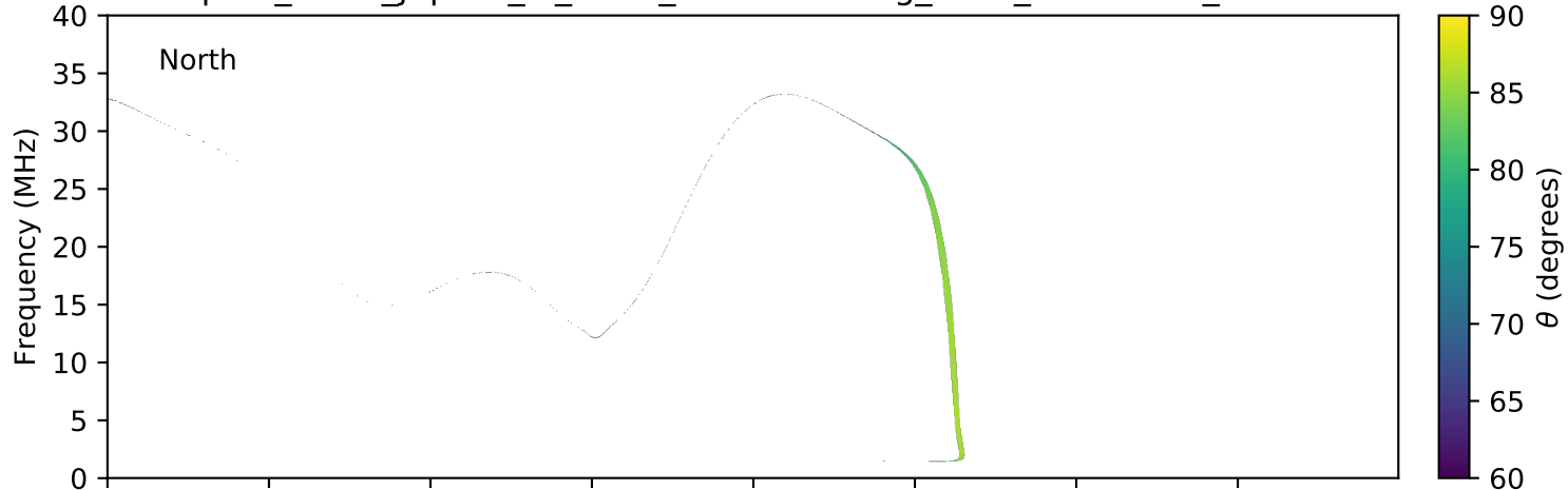
expres_earth_jupiter_io_isaac_lossc-wid1deg_1kev_20161031_v01.cdf
