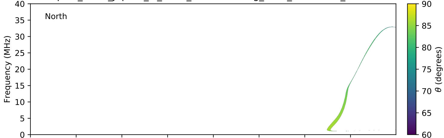
expres_earth_jupiter_io_isaac_lossc-wid1deg_1kev_20161030_v01.cdf
