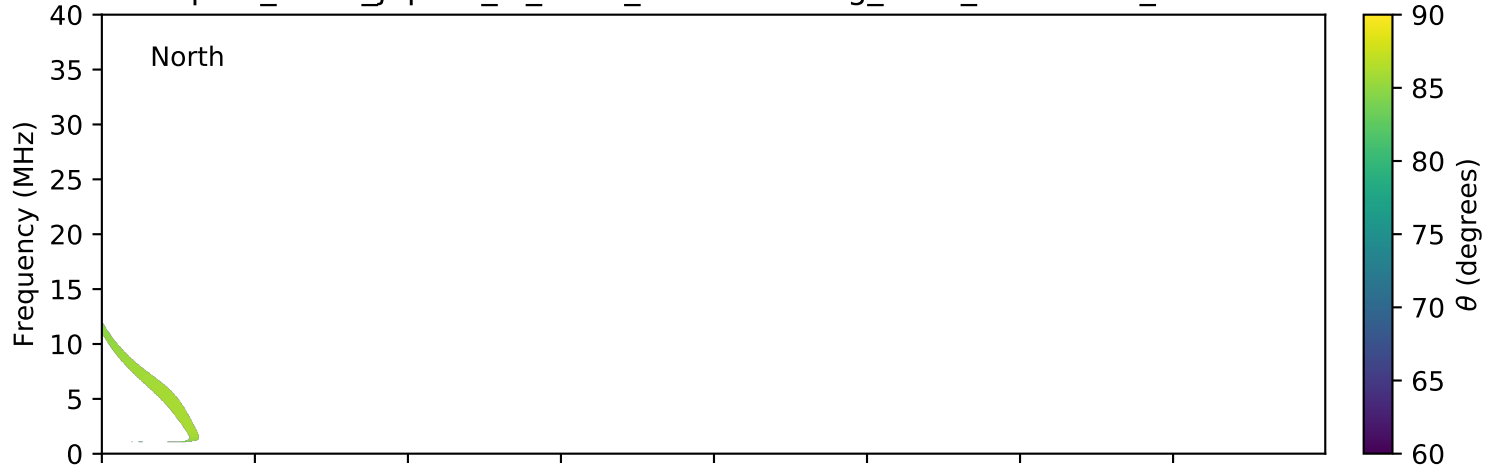
expres_earth_jupiter_io_isaac_lossc-wid1deg_1kev_20161028_v01.cdf
