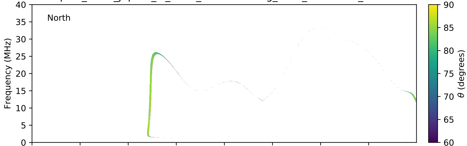
expres_earth_jupiter_io_isaac_lossc-wid1deg_1kev_20161027_v01.cdf
