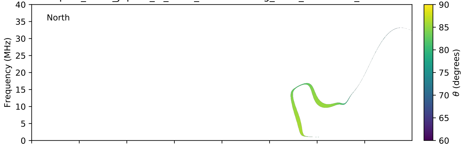
expres_earth_jupiter_io_isaac_lossc-wid1deg_1kev_20161023_v01.cdf
