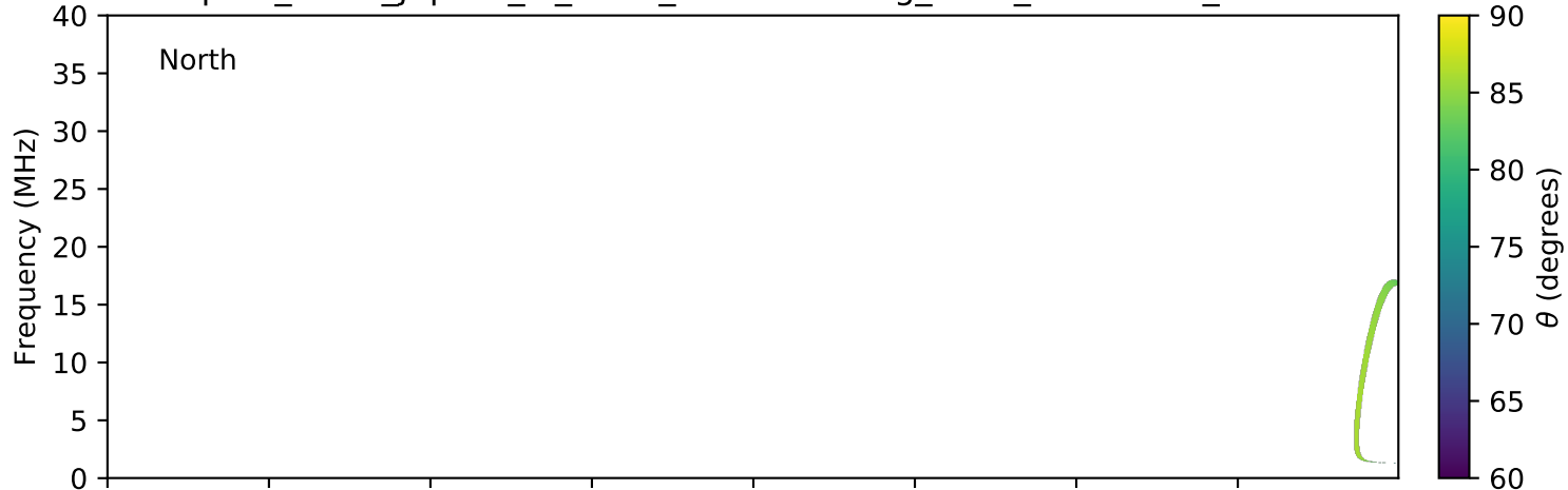
expres_earth_jupiter_io_isaac_lossc-wid1deg_1kev_20161021_v01.cdf
