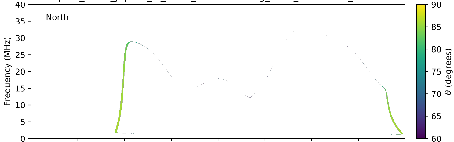
expres_earth_jupiter_io_isaac_lossc-wid1deg_1kev_20161020_v01.cdf
