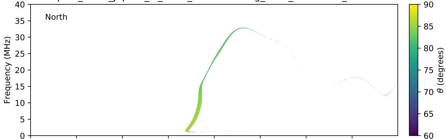
expres_earth_jupiter_io_isaac_lossc-wid1deg_1kev_20161018_v01.cdf
