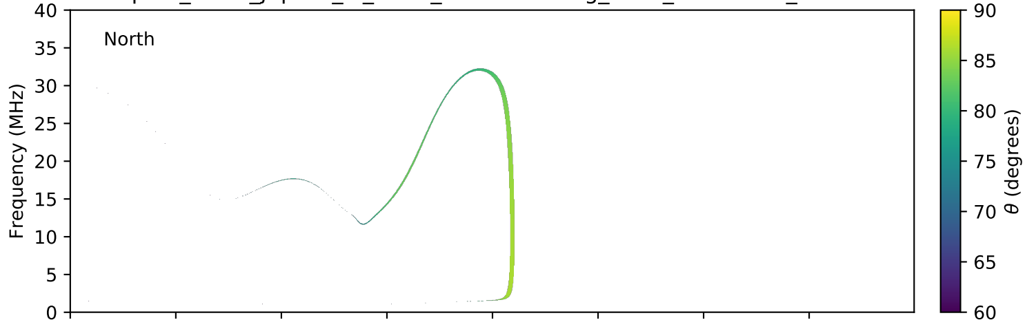
expres_earth_jupiter_io_isaac_lossc-wid1deg_1kev_20161017_v01.cdf
