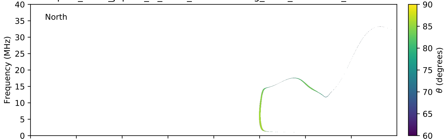
expres_earth_jupiter_io_isaac_lossc-wid1deg_1kev_20161016_v01.cdf
