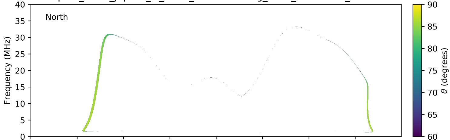
expres_earth_jupiter_io_isaac_lossc-wid1deg_1kev_20161013_v01.cdf
