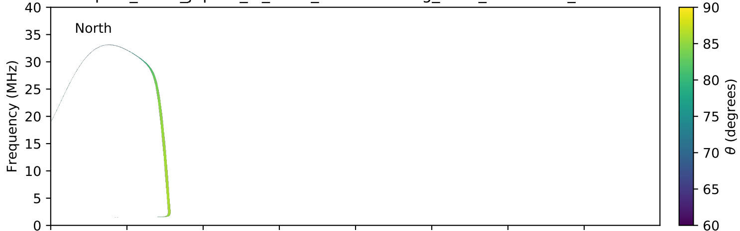
expres_earth_jupiter_io_isaac_lossc-wid1deg_1kev_20161012_v01.cdf
