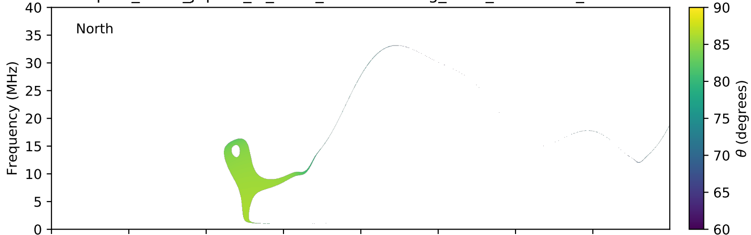
expres_earth_jupiter_io_isaac_lossc-wid1deg_1kev_20161011_v01.cdf
