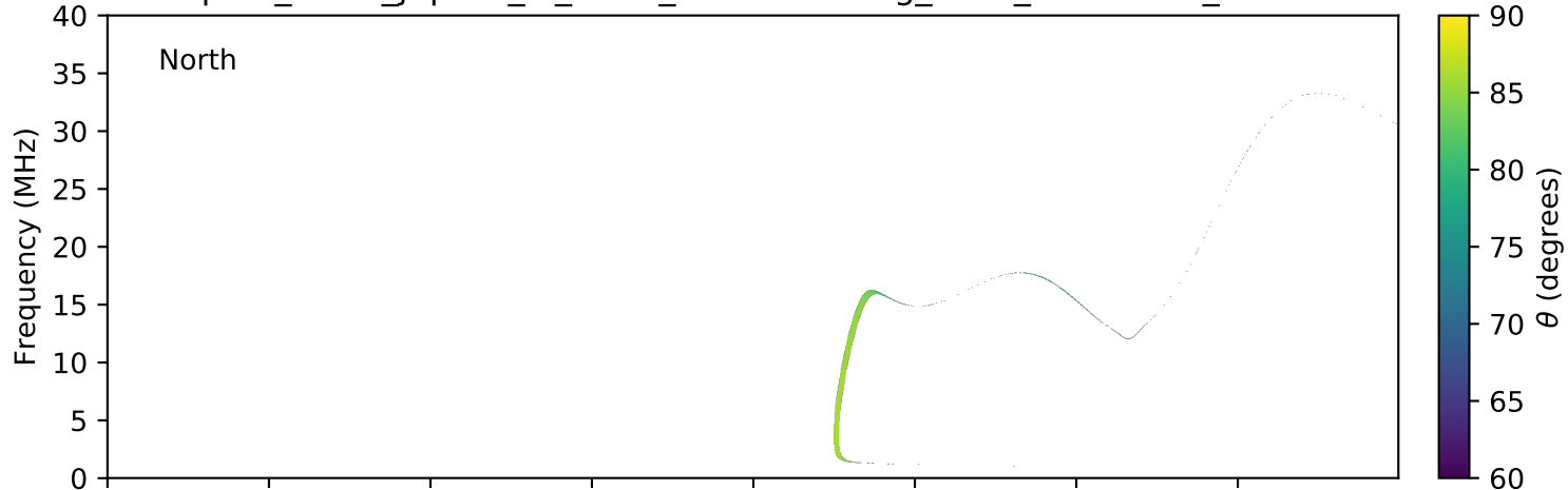
expres_earth_jupiter_io_isaac_lossc-wid1deg_1kev_20161009_v01.cdf
