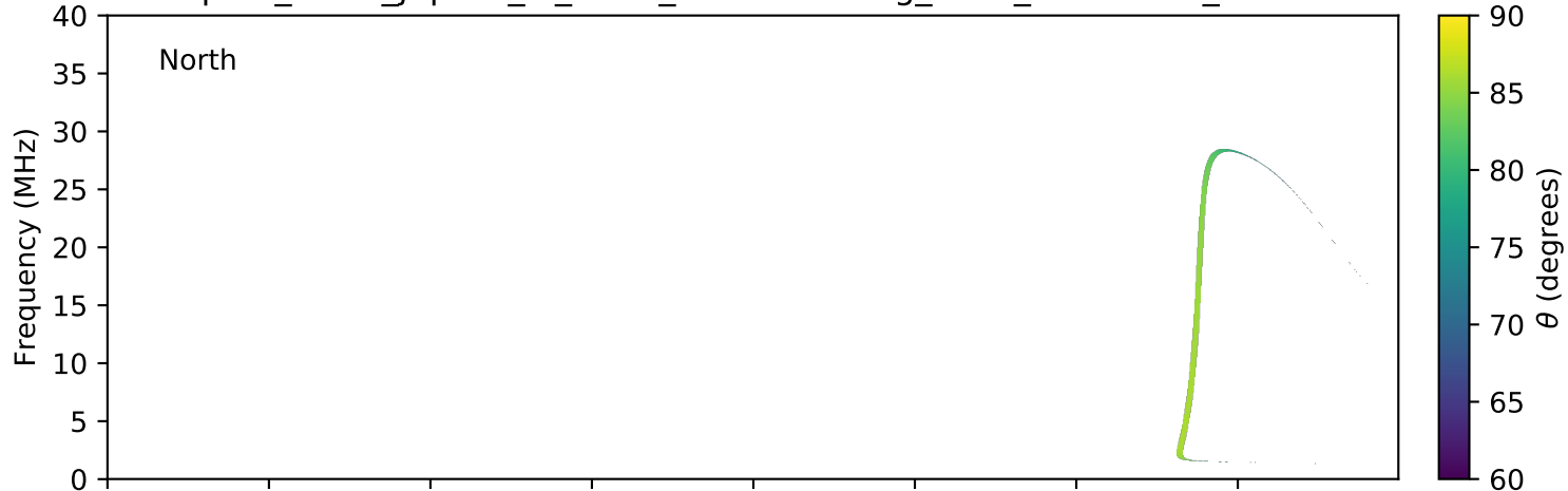
expres_earth_jupiter_io_isaac_lossc-wid1deg_1kev_20161007_v01.cdf
