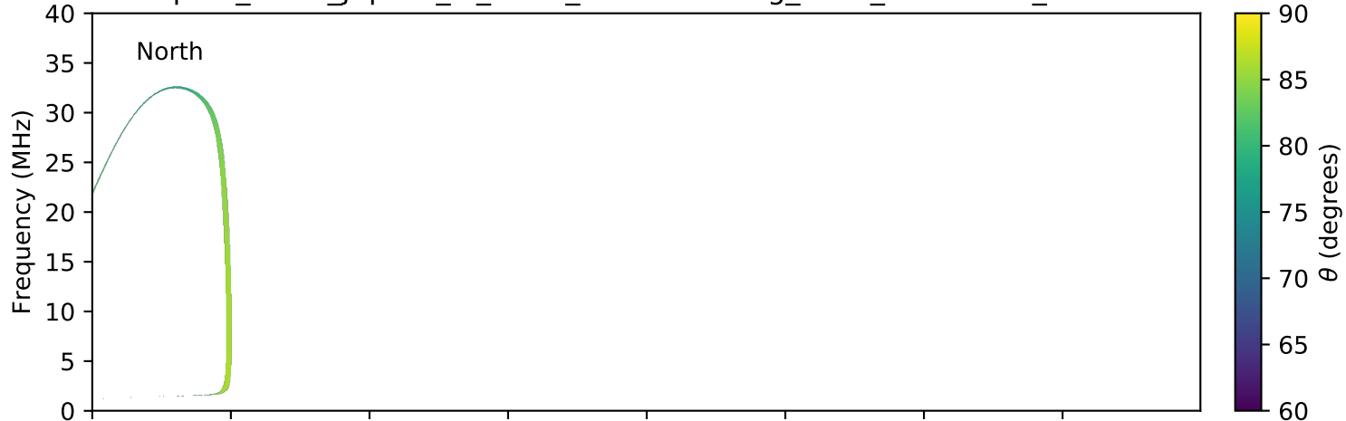
expres_earth_jupiter_io_isaac_lossc-wid1deg_1kev_20161005_v01.cdf
