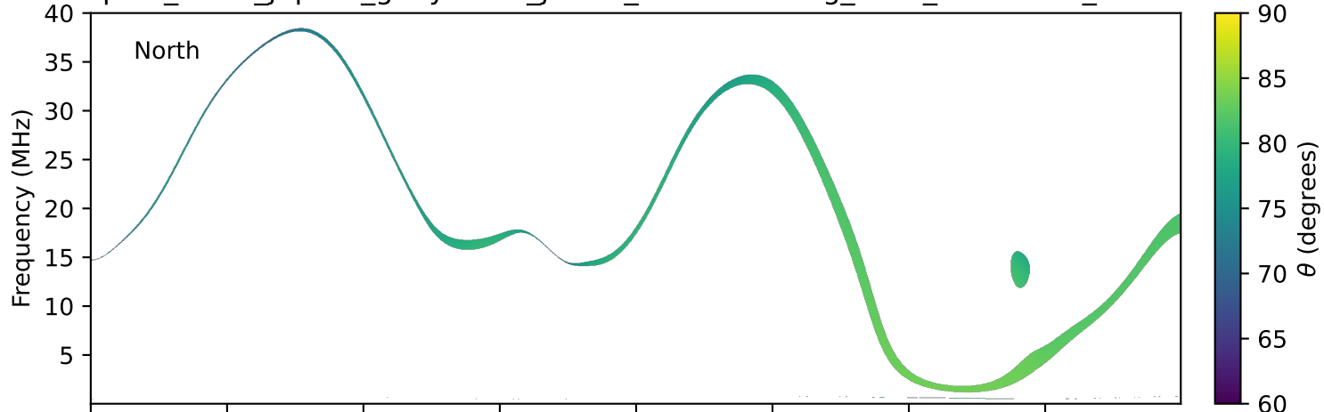
expres_earth_jupiter_ganymede_jrm33_lossc-wid1deg_3kev_20161014_v11.cdf
